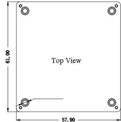
Standard 61*57.9*12.7mm
