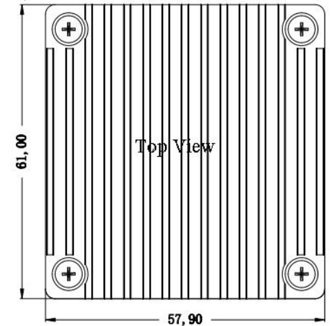
Standard+Heatsink 61*57.9*27.7mm
