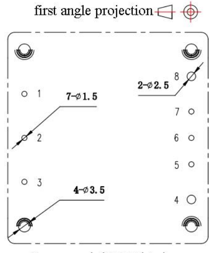
Recommended PCB Slot size
